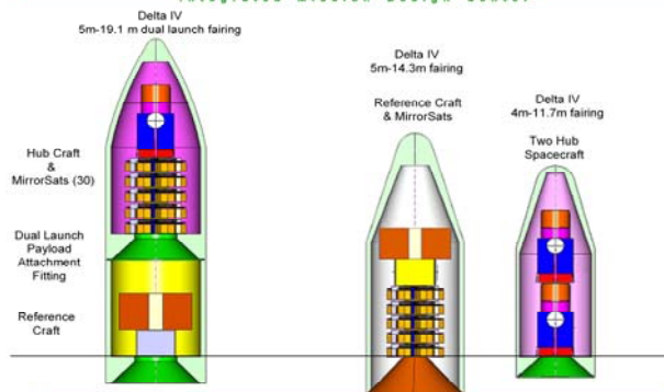
Fig. 9: Two launch options for SI, a single Delta IV heavy vs. two Delta IV launches
