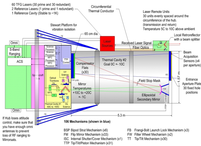
Fig. 7: A detailed look at the hub design, showing optics, detectors, metrology components, and support systems.
