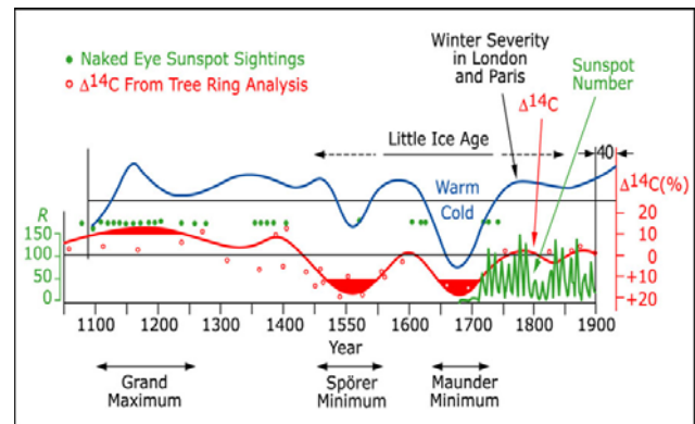
Fig. 2: Short term variations in solar activity and their impact on Earth
