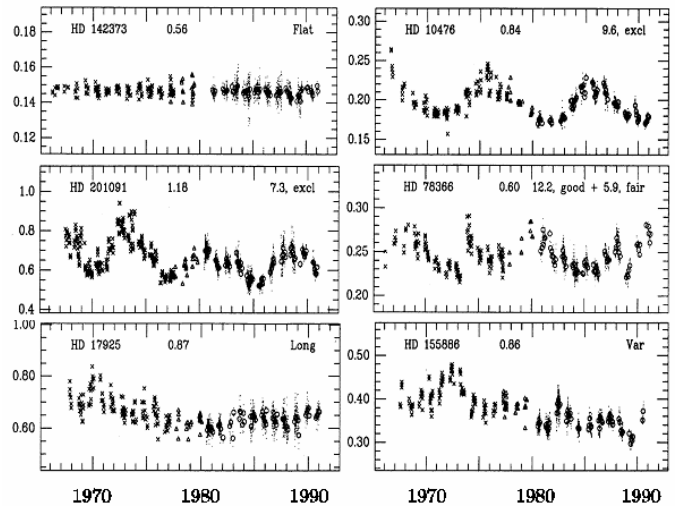
Fig. 1: Records of the relative Ca II H+K fluxes of main-sequence stars: x, Wilson's records (1966–1977); triangles and dots, Ca II HK survey (1977–1992); open circles 30-day averages. The top of each panel shows the stellar identification, color index B–V, and a classification of the long-term variability or period(s) in case of cyclic activity (figure from Baliunas et al., 1995).
