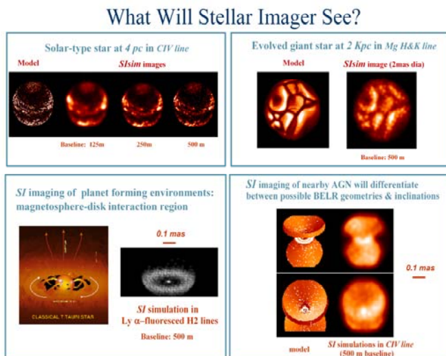
Fig. 3: Simulations of some of SI's capabilities for UV imaging, assuming 30 mirror elements in a non-redundant pattern.
