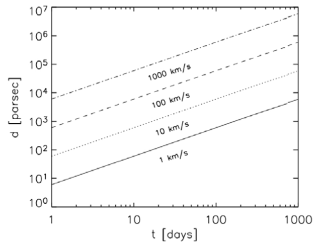
Fig. 4: Minimum time interval between successive SI images required to resolve the motion of a feature moving at different speeds (line labels) as a function of the object's distance.
